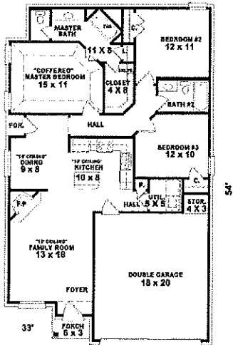
ORIGINALLY PROPOSED FLOOR PLAN
